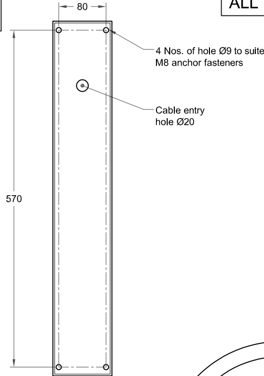
Mounting Detail Scale: 1.5 : 1
