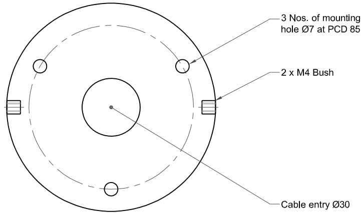
Mounting Detail scale: 2 : 1
